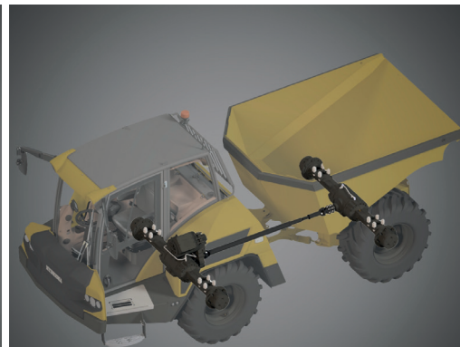
ZF eTrac Driveline
